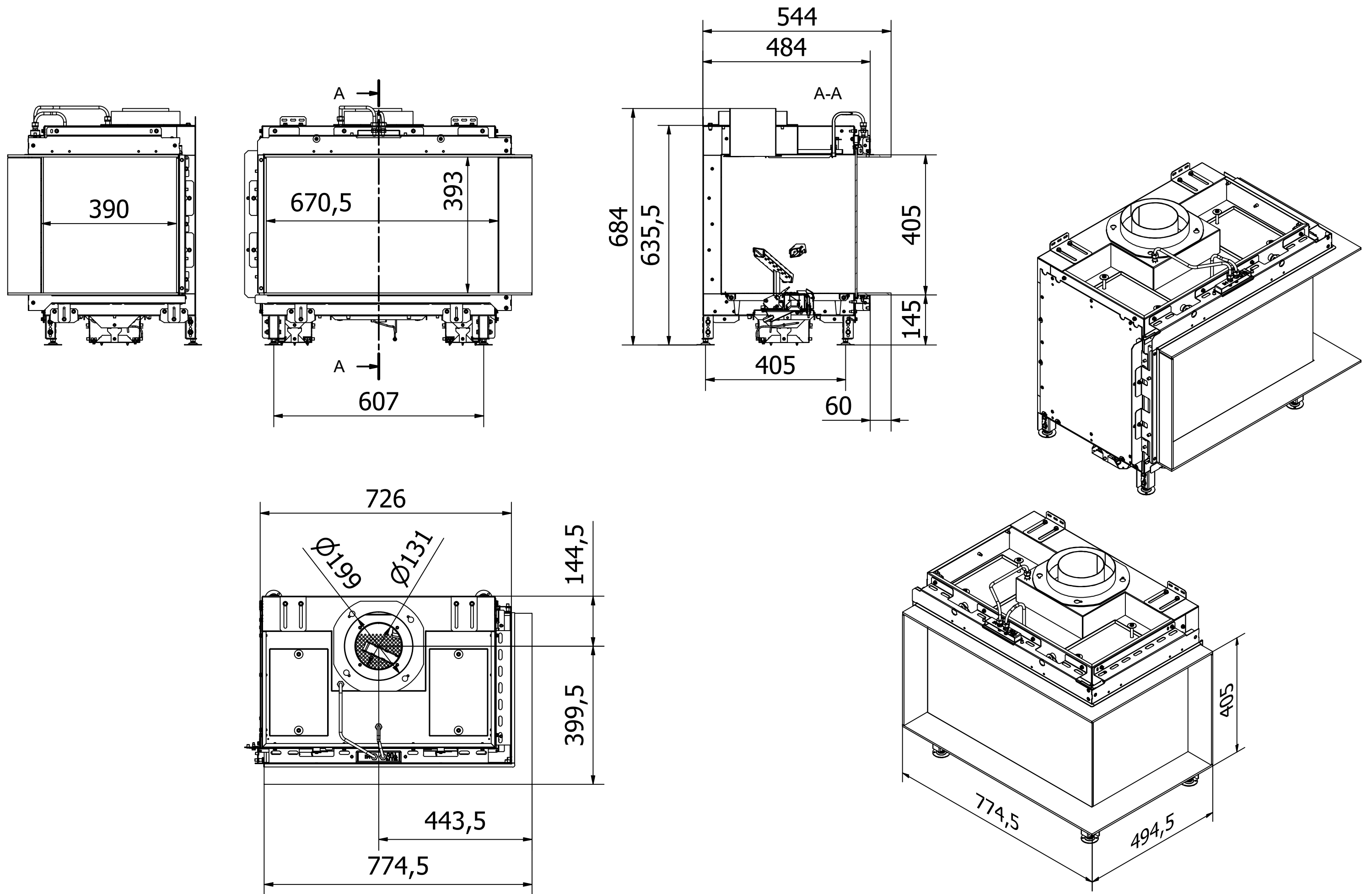
RAIS Visio Gas 70-43-39 RC-6541
